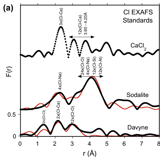
Fig. 5a. Partial RDFs of the standards, CaCl_2 , sodalite, and davyne with pair correlations indicated for the major features. Final fits from FEFFIT (red lines) for sodalite and davyne are indicated. Plots are offset for clarity. (For interpretation of the references to colour in this figure legend, the reader is referred to the web version of this article.)
